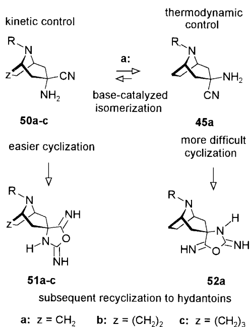
Scheme 4 Origin of the complementarity of formation of troponespirohydantoin diastereomers
