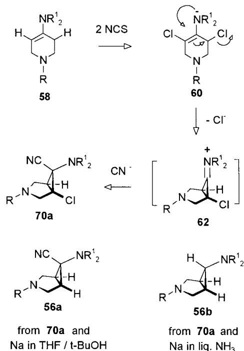
Scheme 11 Dichloroenamines as access to 6\alpha -amino-3-azabicyclo[3.1.0]hexane derivatives
