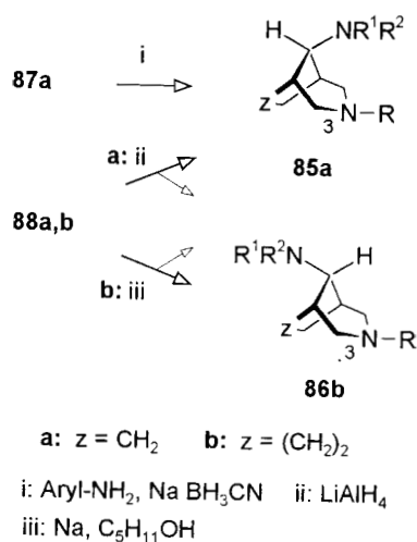
Scheme 12 Diastereoselective routes to amines of norcamphidine and its homologues
