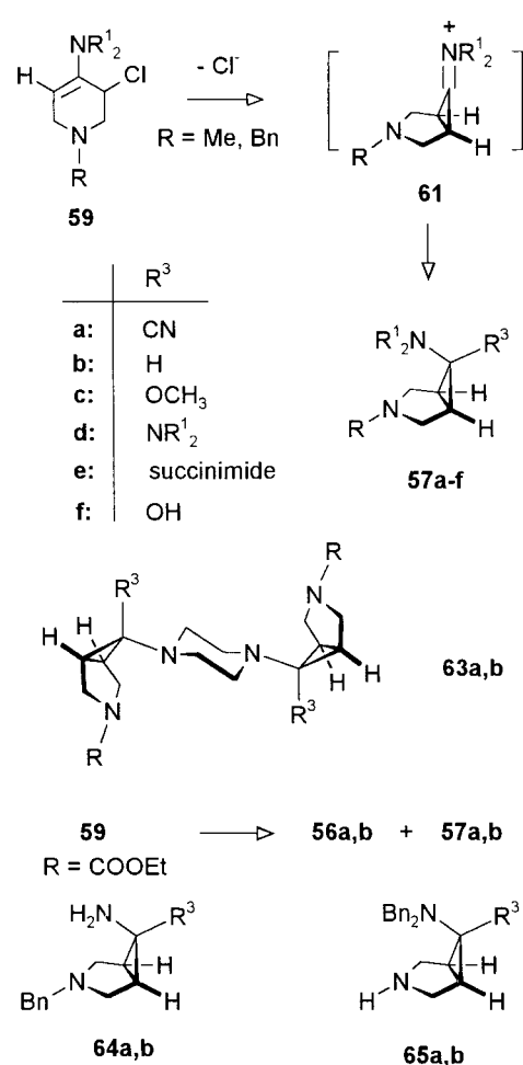
Scheme 6 6β-Amino-3-azabicyclo[3.1.0]hexane derivatives from chloroenamines
